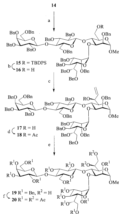
Scheme 3. a) 1. MeOH/Et 3 N/water (2:1:1, v/v/v), room temp.; 2. BnBr, NaH, DMF, molecular sieves (4 Å), DMF, 0 °C → room temp., 69%; b) TBAF, THF, room temp. → 60 °C, 89%; c) 1. (COCl) 2 , DMSO/THF, -60 °C, then Et 3 N; 2. CH 2 =CHMgBr, THF, -70 °C, 78%; d) Ac 2 O, DMAP, pyridine, 82%; e) 1. OsO 4 /NaIO 4 , Et 2 O/water (1:1, v/v), 30–35 °C; 2. NaBH 4 , DMF/MeOH (2:1, v/v), 80%; f) 1. H 2 , Pd/C, EtOH/AcOH/water (7:5:5, v/v/v); 2. Ac 2 O, DMAP, pyridine, 84%
