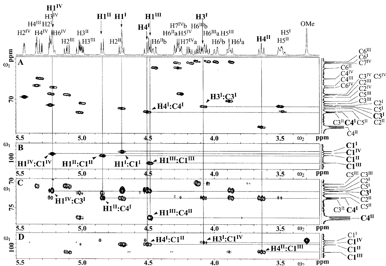
Figure 2. Partial HMQC (panels A and B) and HMBC (panels C and D) spectra of compound 14 recorded in \text{CDCl}_3 at 25 °C; only partial ^{13}\text{C}/^1\text{H} cross-peaks (A and B) and cross-relay peaks (C and D) are labeled; each Roman numeral in panels A–D corresponds to that of 14 as shown in Scheme 2
