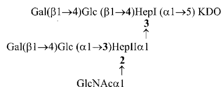
Figure 1. The oligosaccharide structure of LOS produced by Neisseria gonorrhoeae strain 15253; Gal: D -galactose; Glc: D -glucose; Hep: L -glycero- D -manno-heptose; GlcNAc: N -acetyl- D -glucosamine; KDO: 2-keto-3-deoxy- D -manno-octulosonic acid; the two heptoses are designated as described previously [8]
