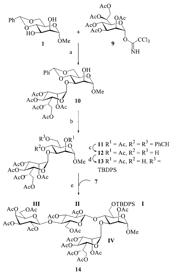
Scheme 2. a) \text{BF}_3 \cdot \text{OEt}_2 , \text{CH}_2\text{Cl}_2 , -10^\circ\text{C} , 70%; b) \text{Ac}_2\text{O} , DMAP, pyridine, 89%; c) \text{AcOH} (70% aq.), 70^\circ\text{C} , 93%; d) TBDPSCl, imidazole, DMF, room temp., 87%; e) \text{BF}_3 \cdot \text{OEt}_2 , \text{CH}_2\text{Cl}_2 , -10^\circ\text{C} \rightarrow room temp., 59%
