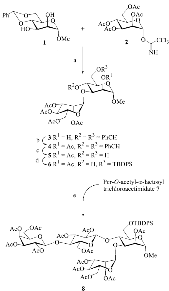
Scheme 1. a) \text{BF}_3 \cdot \text{OEt}_2 , \text{CH}_2\text{Cl}_2 , -10^\circ\text{C} , 56%; b) \text{Ac}_2\text{O} , pyridine, 99%; c) \text{AcOH} (70% aq.), 60-70^\circ\text{C} , 93%; d) TBDPSCl, imidazole, DMF, 0^\circ\text{C} \rightarrow \text{room temp.} , 93%; e) \text{BF}_3 \cdot \text{OEt}_2 , \text{CH}_2\text{Cl}_2 , -10^\circ\text{C} , 80%
